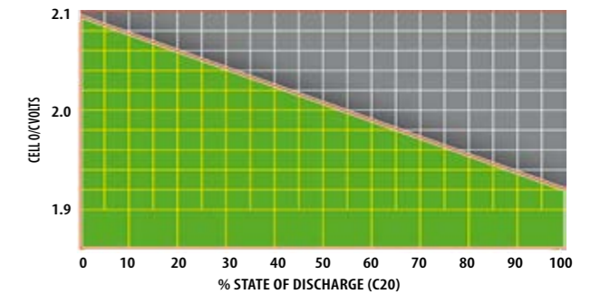
Open Circuit Voltage VS Discharge Depth for Energystore
